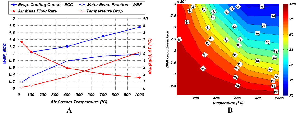
Figure 4. A. Various resulting parameters due temperature change at the inlet. B. Evaporation percentage that is inside spray plume defined by variable DPM concentration.
