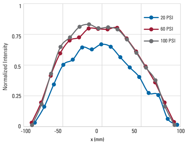
FIGURE 7: HHX FullJet nozzle distributions at various pressures
