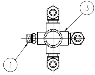
SECTION A'-A' SCALE 3:1
