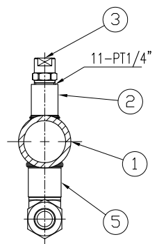
SECTION "A"-"A" (SCALE 3:1)
