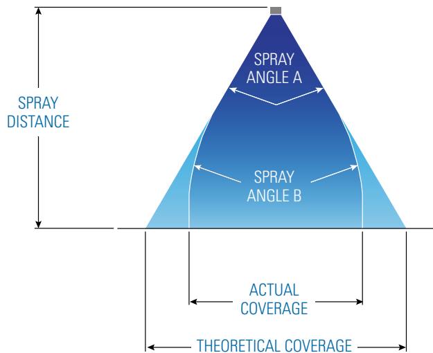
Spray Angle "A" is measured close to the orifice. Theoretical coverage at a specific spray distance can be calculated from this angle. Spray Angle "B" is measured from actual coverage at a particular spray distance. For SprayDry® nozzles, the "B" angles are measured 12 inches (30.5 cm) from the nozzle orifice.
