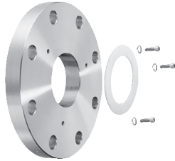
Mounting kit for mounting the standard AA190 three-prong flange to a 4" 150# flange Includes 316 Stainless Steel raised face flange, lockwasher, bolts and PTFE gasket
