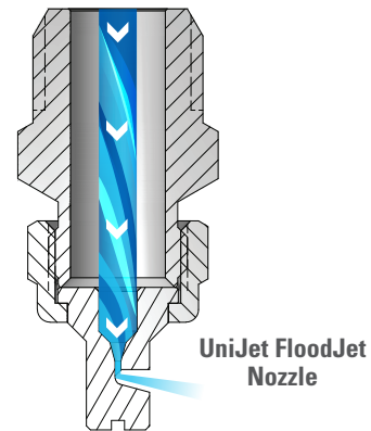
UniJet FloodJet® Nozzles
